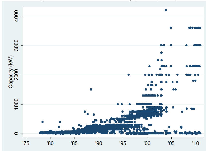
Figure 3: Installed Turbine Size (by rated power)
