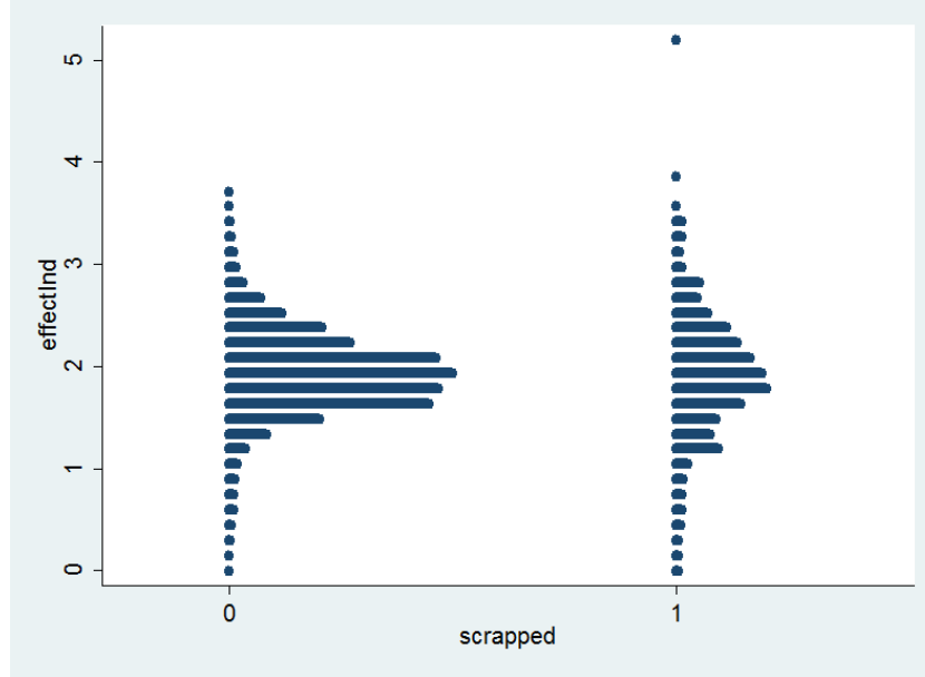
Figure 10: Dot Plot of Turbine Efficiency Indicator
